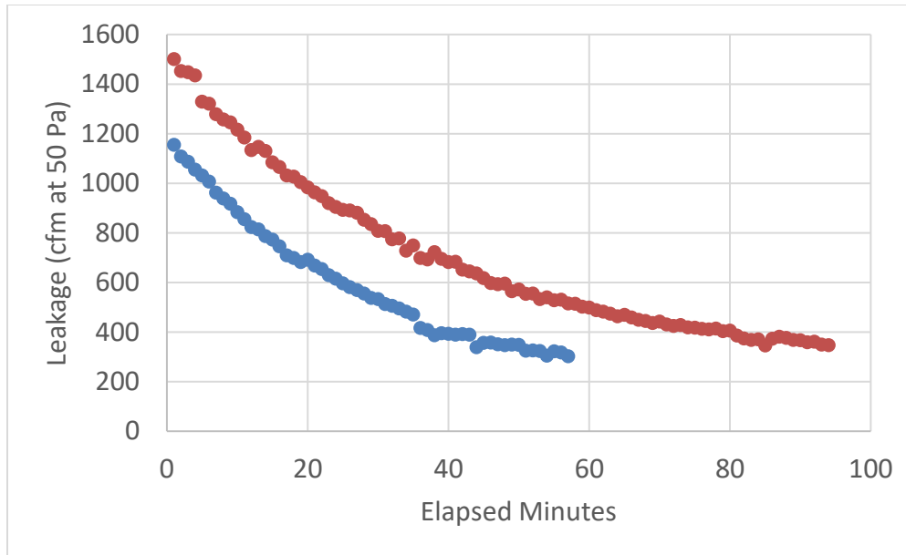
Figure 4. Sealing profile for both houses sealed under Option 1
