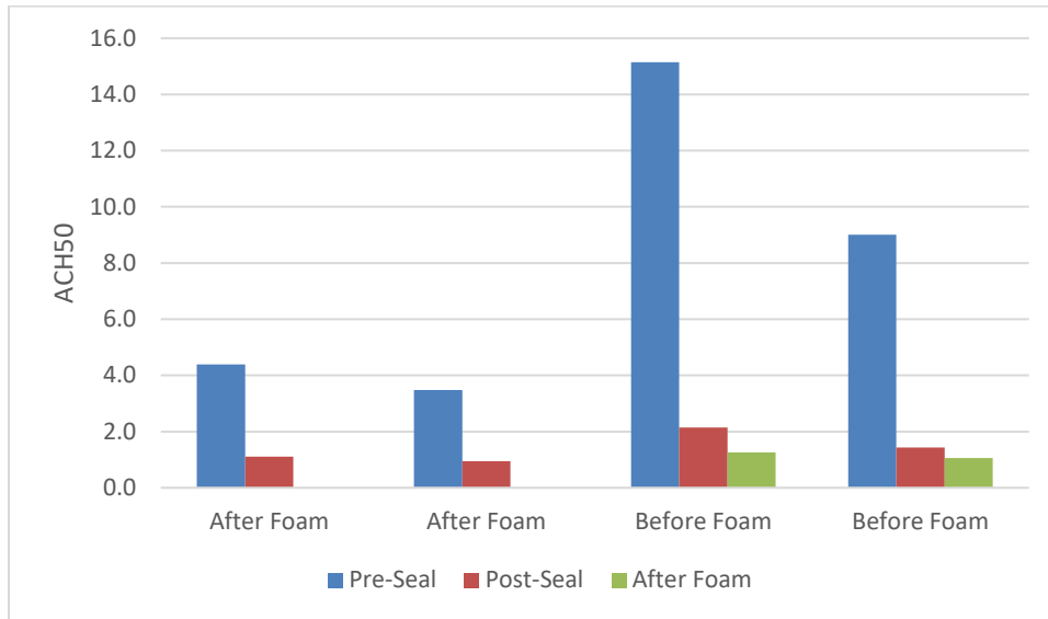
Figure 11. Air leakage results summary for all homes at each stage of process
