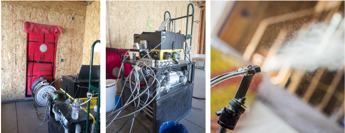
Pressurization fan installed in garage door
