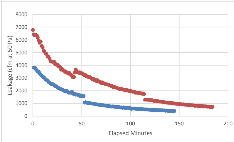
Figure 10. Sealing profile for both houses sealed under Option 2
