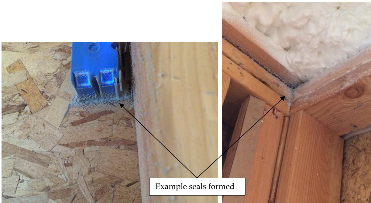
Figure 6. AeroBarrier seals formed at exterior electrical outlet and corner of wall assembly
